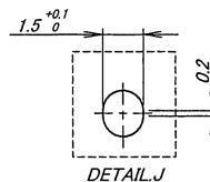
DETAIL J
