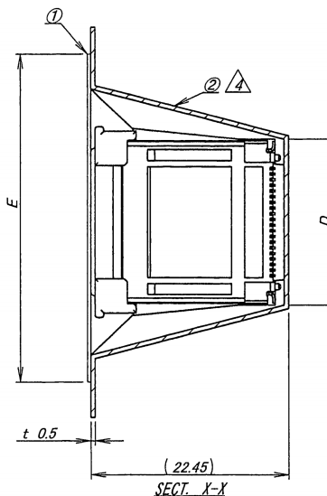
SECT. X-X
