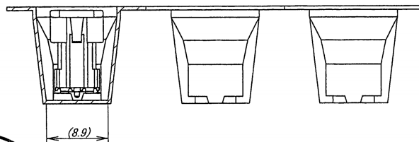
SECT. Y-Y
