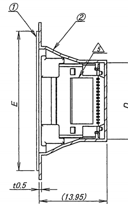
SECT. X-X
