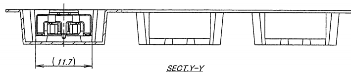
SECT.Y-Y
