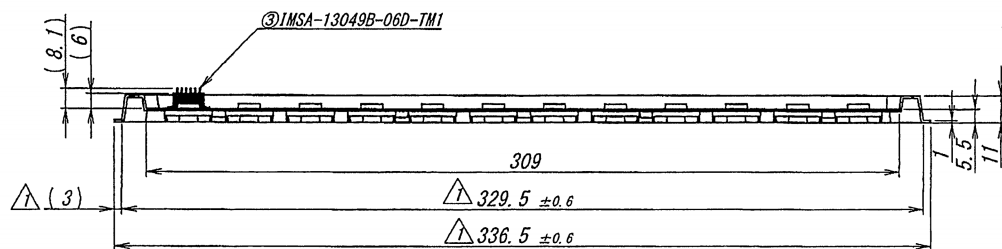
SECT. B-B
