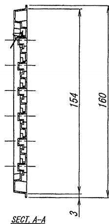
SECT. A-A
