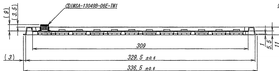
SECT. B-B
