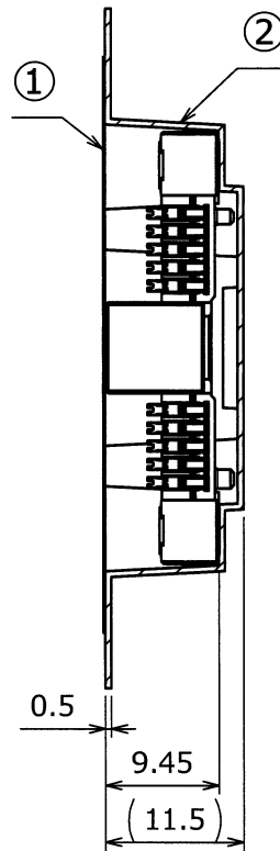
SECT B-B
