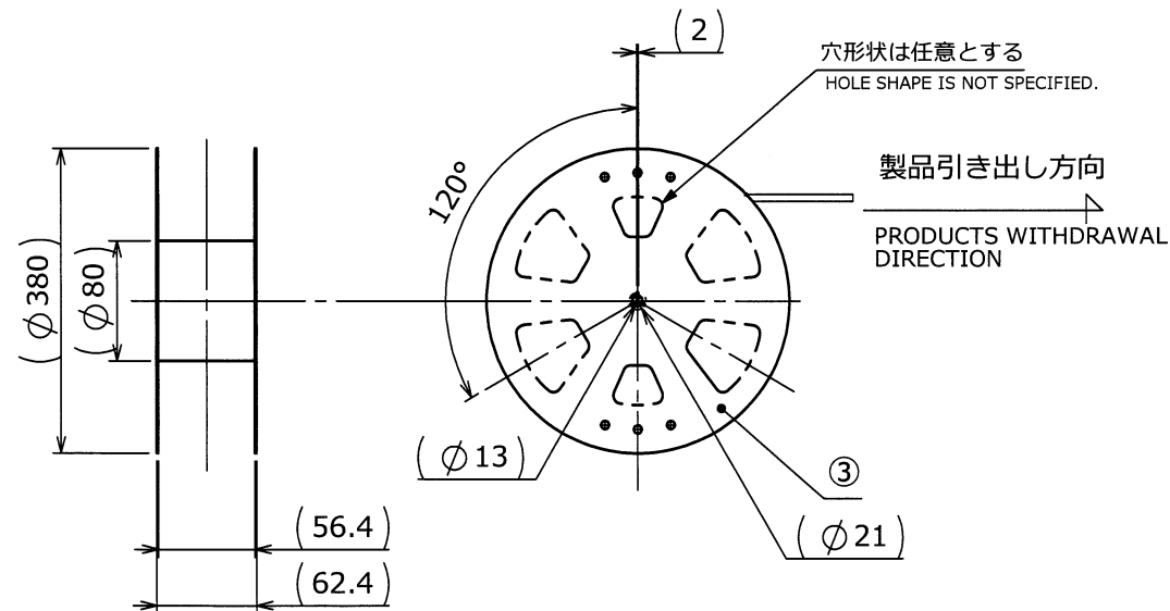
SECT B-B
