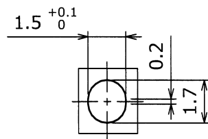
DETAIL C
