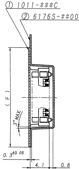
SECT. H-H
