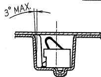
SECT. G-G
