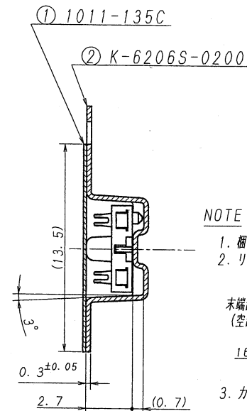
SECT. A-A
