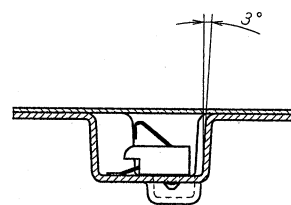
SECT. B-B
