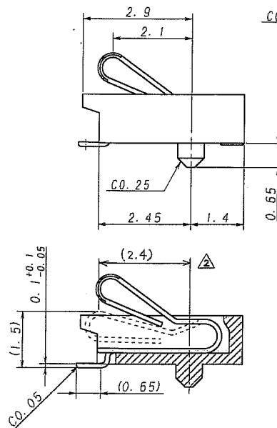
SECT. A-A
