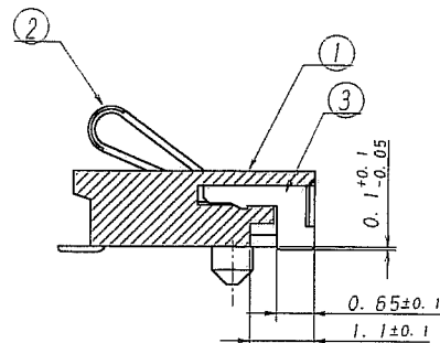
SECT. B-B
