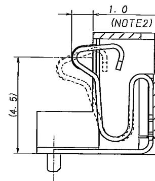
SECT. A-A
