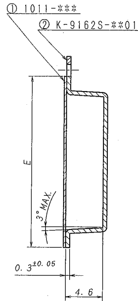
SECT. G-G
