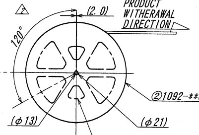
SECT. J-J
