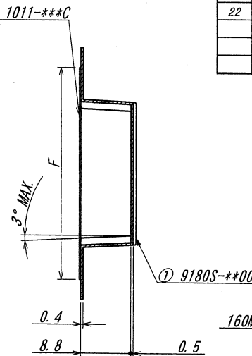
SECT. J-J
