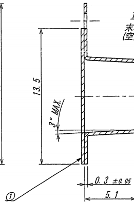
SECT. B-B
