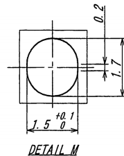
DETAIL M
