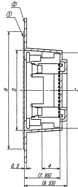
SECT. L-L
