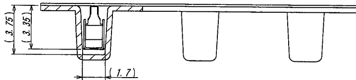
SECT. B-B
