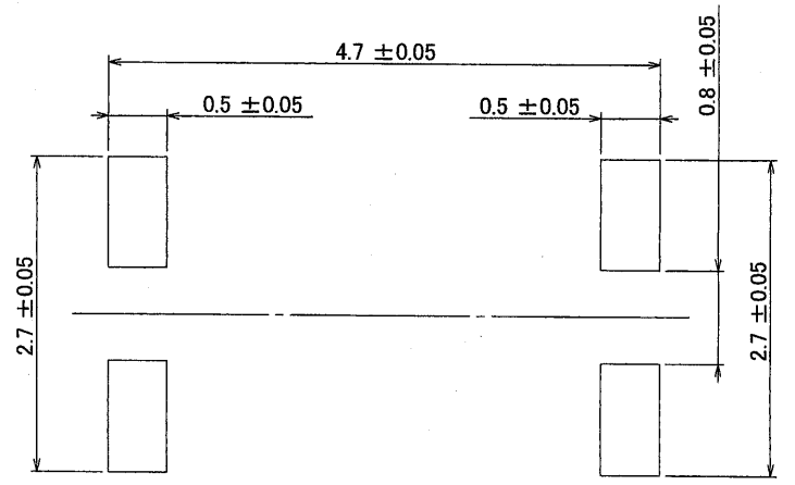
推奨基板パターン/RECOMMENDED PCB PATTERN
