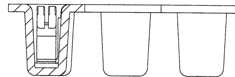
SECT B-B
