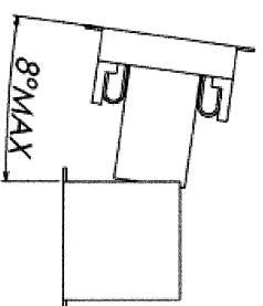
図2/ Fig.2 (垂直接続タイプに適用/ Apply to vertical connection)
